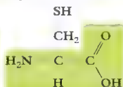
cysteine (Cys) C 5,02
